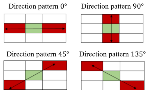
Figure 4 Image of dividing the range of the color change direction by the image.
