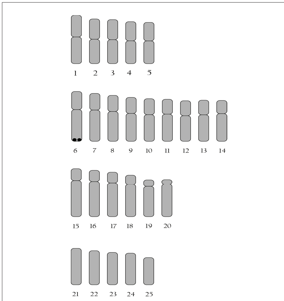
Figure 4. The standardize idiogram of Lobocheilos rhabdoura showing lengths and shapes of chromosomes ( n = 25 ) by NOR-banding technique. Black dots indicate telomeric NOR-bearing chromosome pair 6.
