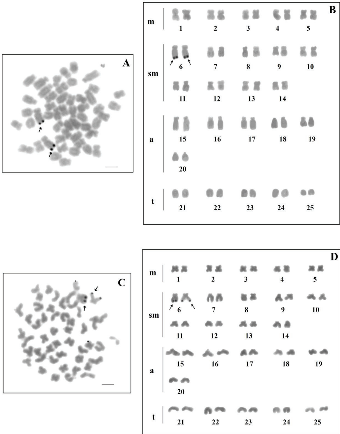
Figure 3. The metaphase chromosome plates and karyotypes of male (A, B) and female (C, D) of Lobocheilos rhabdoura (2n=50) by NOR-banding technique. Scale bars indicate 2 μm. (Arrows indicate NORs)
