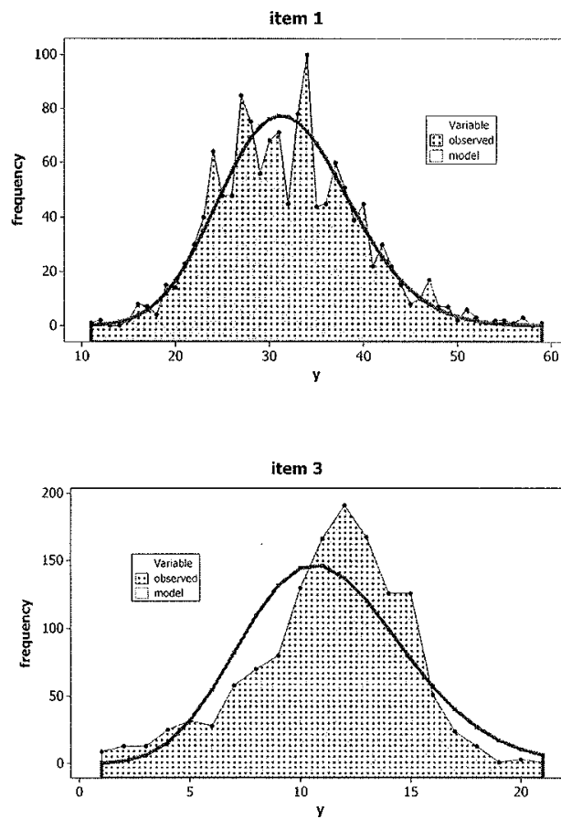
Figure 4: Covariate adjusted frequency plots for the RPCM for items 1 and 3 measuring processing speed.
