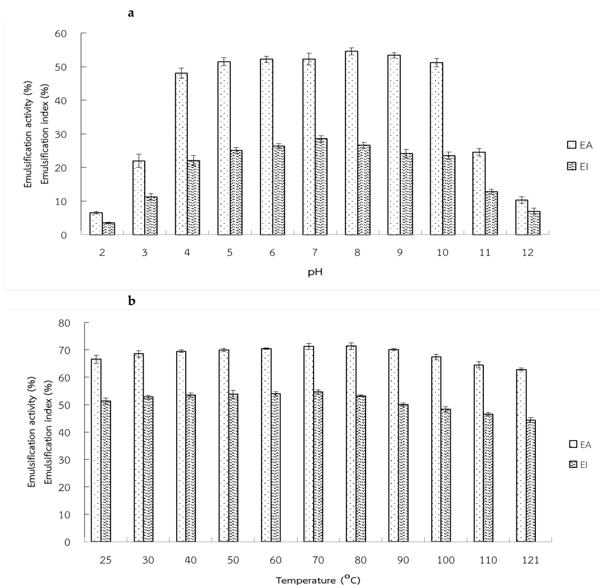
Figure 2. Effect of pH (a) and temperature (b) on emulsion activity of crude biosurfactant produced by B. oceanisediminis PM 08.
