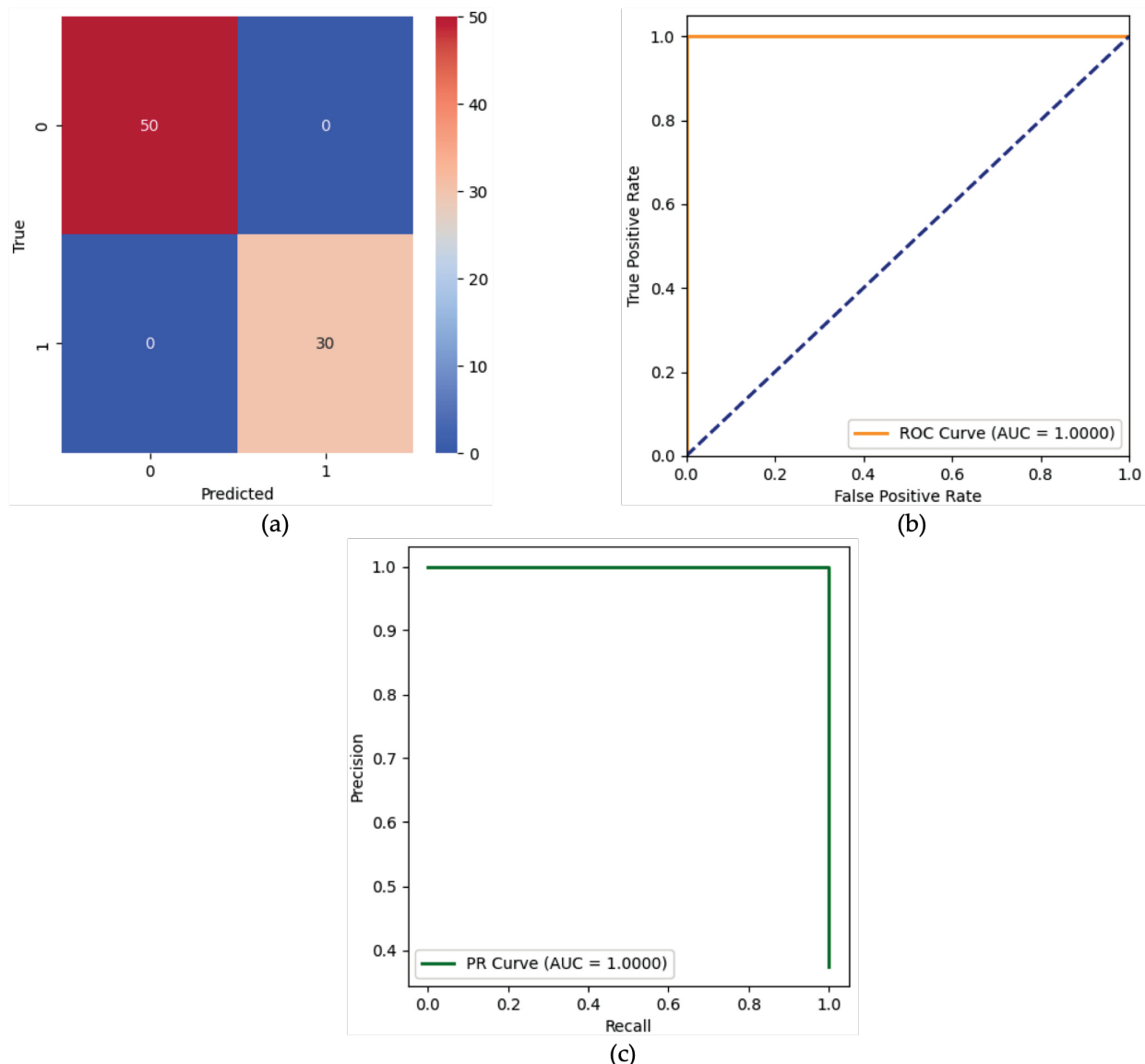
Figure 2. (a) Confusion Matrix, (b) AUROC, (c) AUPRC of GBM on the slightly imbalanced dataset.
