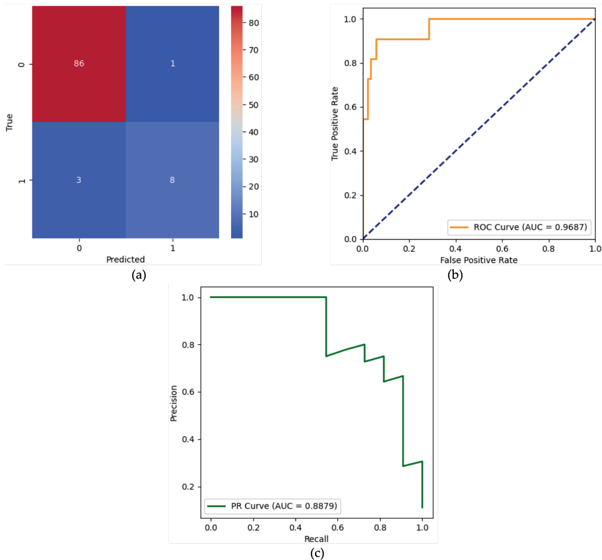
Figure 3. (a) Confusion Matrix, (b) AUROC, (c) AUPRC of GBM on a severely imbalanced dataset.
